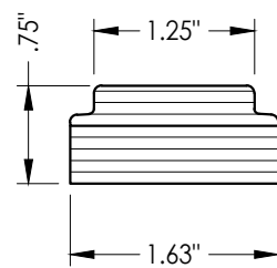
52 SIDELITE TOP RAIL
