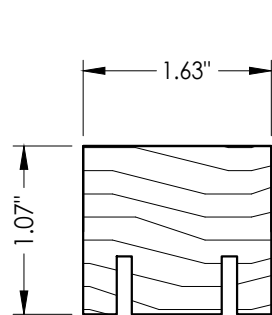
49 SIDELITE BOTTOM RAIL
