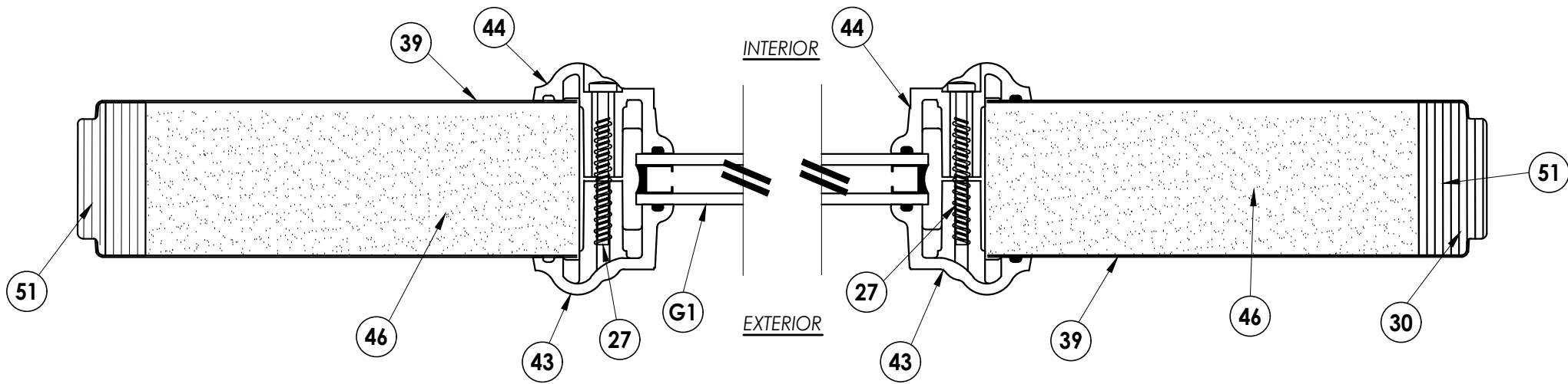
1 3 HORIZONTAL CROSS SECTION
