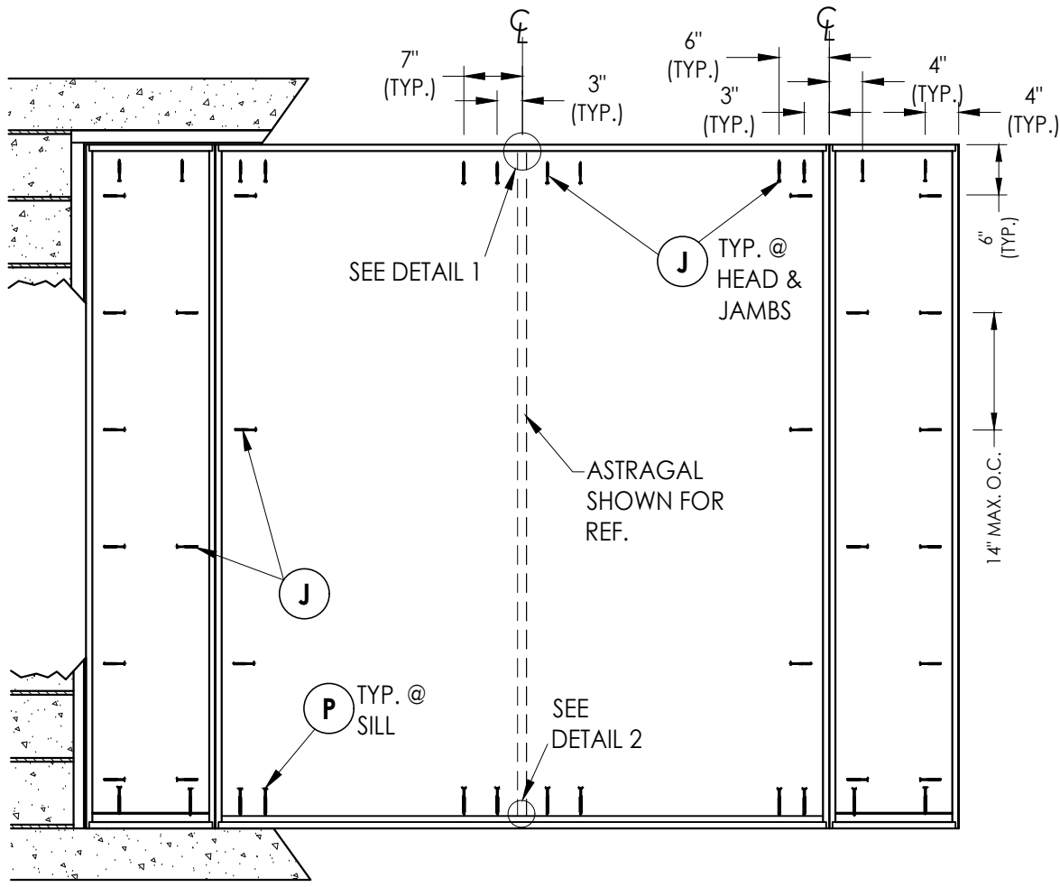
FRAME ANCHORING Masonry 2X buck construction
