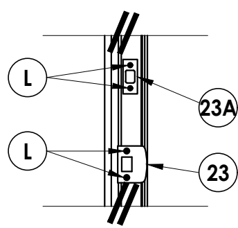
ASTRAGAL DETAIL @ Strike
