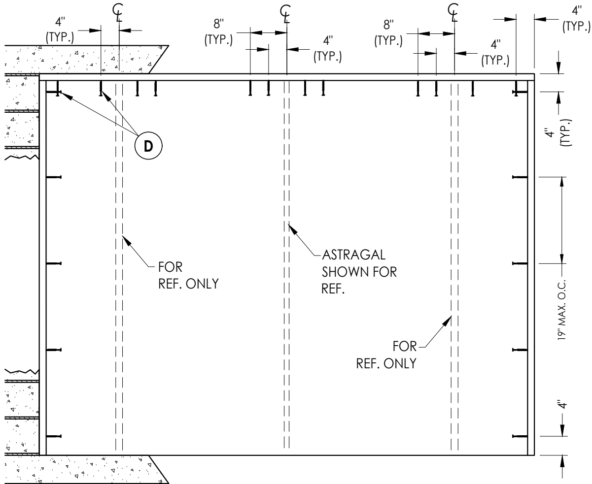
BUCK ANCHORING
